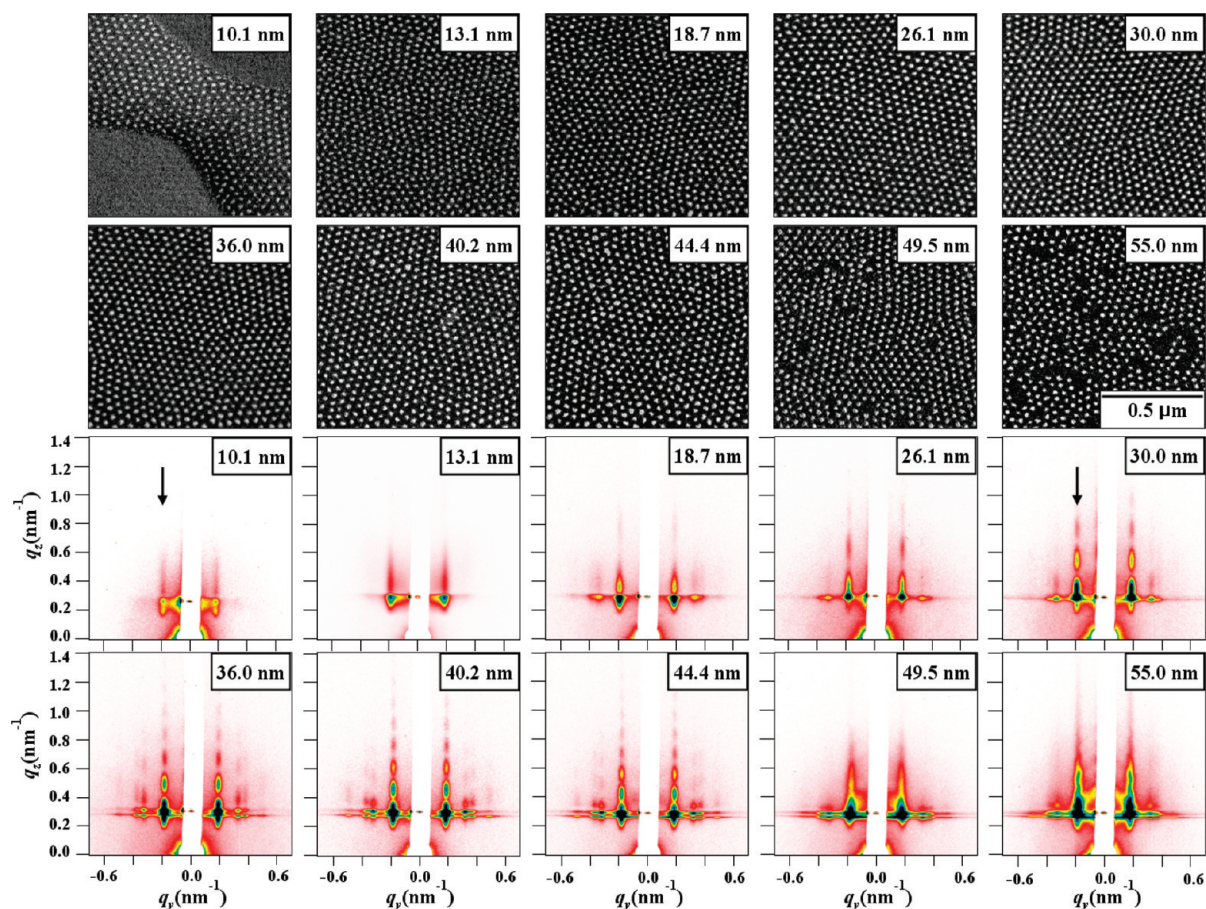
Figure 1. SFM phase images and the corresponding two-dimensional GISAXS patterns at incident angles of 0.16° (10.1 nm thickness) and 0.18° (the others) for thin films of cylinder-forming PS- b -PMMA-80 on the substrate modified by R64 (having a PS mole fraction of 0.64) at various film thicknesses after thermally annealing thin films at 170 °C for 24 h. To increase the scattering contrast, PMMA microdomains were removed from all thin film samples by UV exposure and subsequent rinsing with acetic acid. Arrows are drawn to compare the peak maxima.
